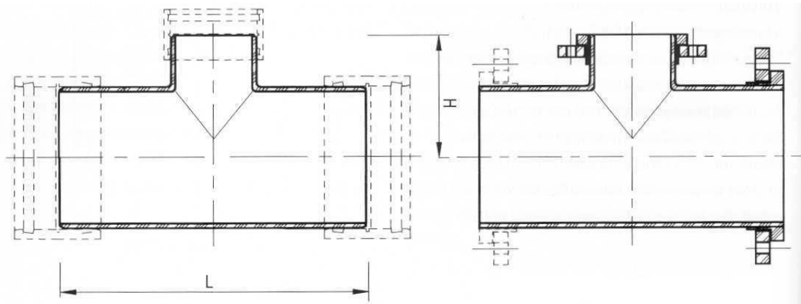
Ταυ ευθέων άκρων
